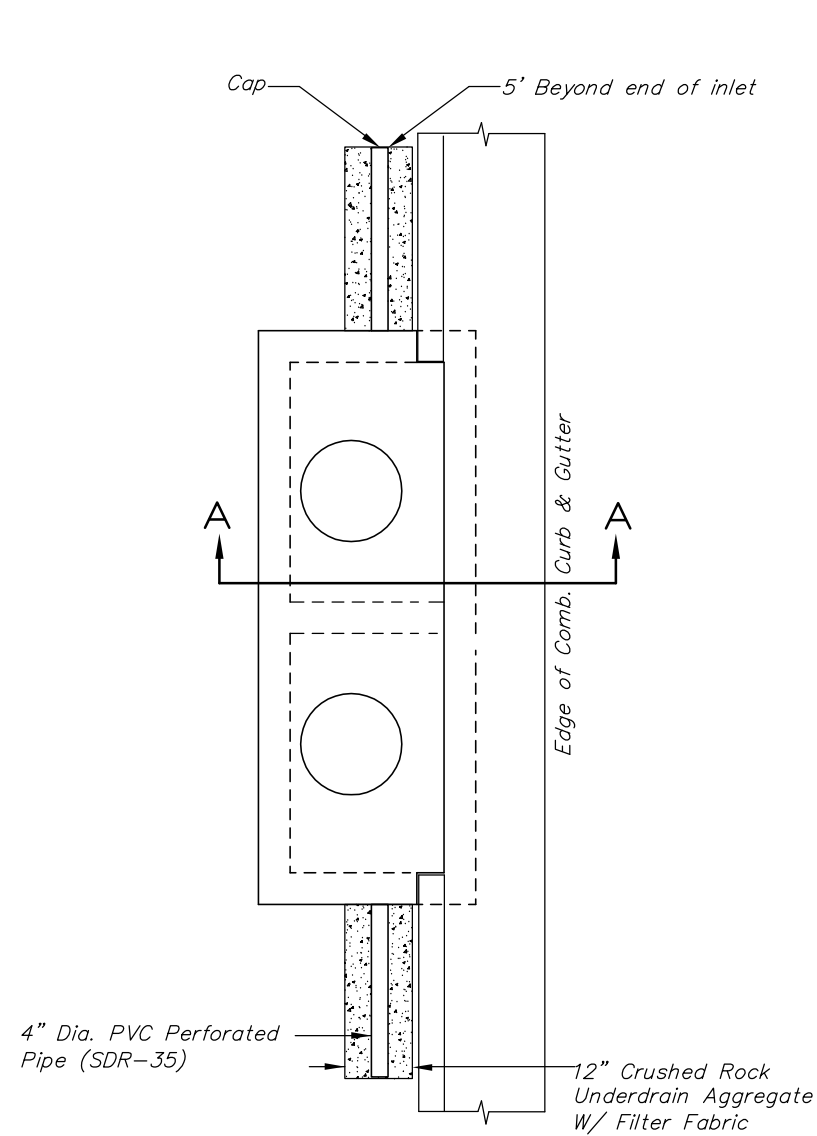
TYPE 1 AND 2 INLET
