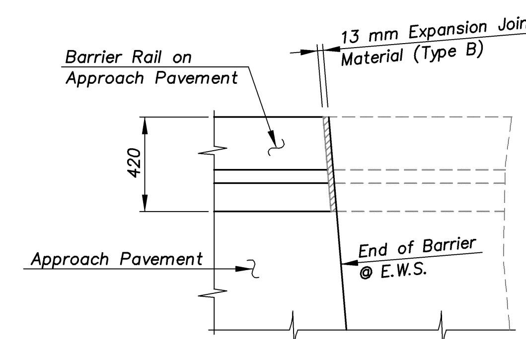
DETAIL "B"
