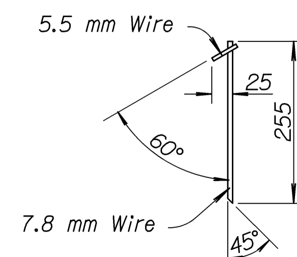
STAKE DETAIL
