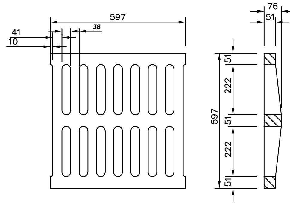
GRATE 24" x 24" FRAME & GRATE DETAIL
