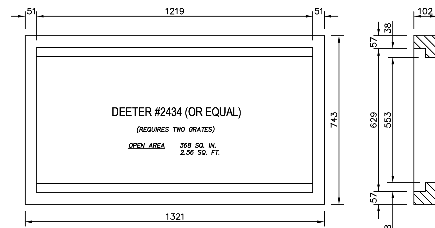
DOUBLE 24" x 24" FRAME DETAIL
