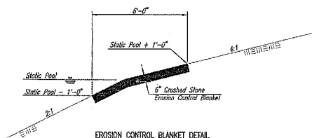
EROSION CONTROL BLANKET DETAIL
