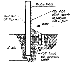
SILT FENCE BARRIERS
