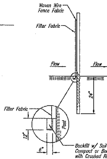
ANCHOR TRENCH DETAIL
