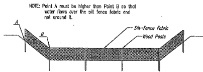
ELEVATION SILT FENCE DITCH CHECKS (STREAM PROTECTION)
