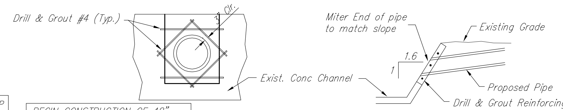
CHANNEL SECTION
