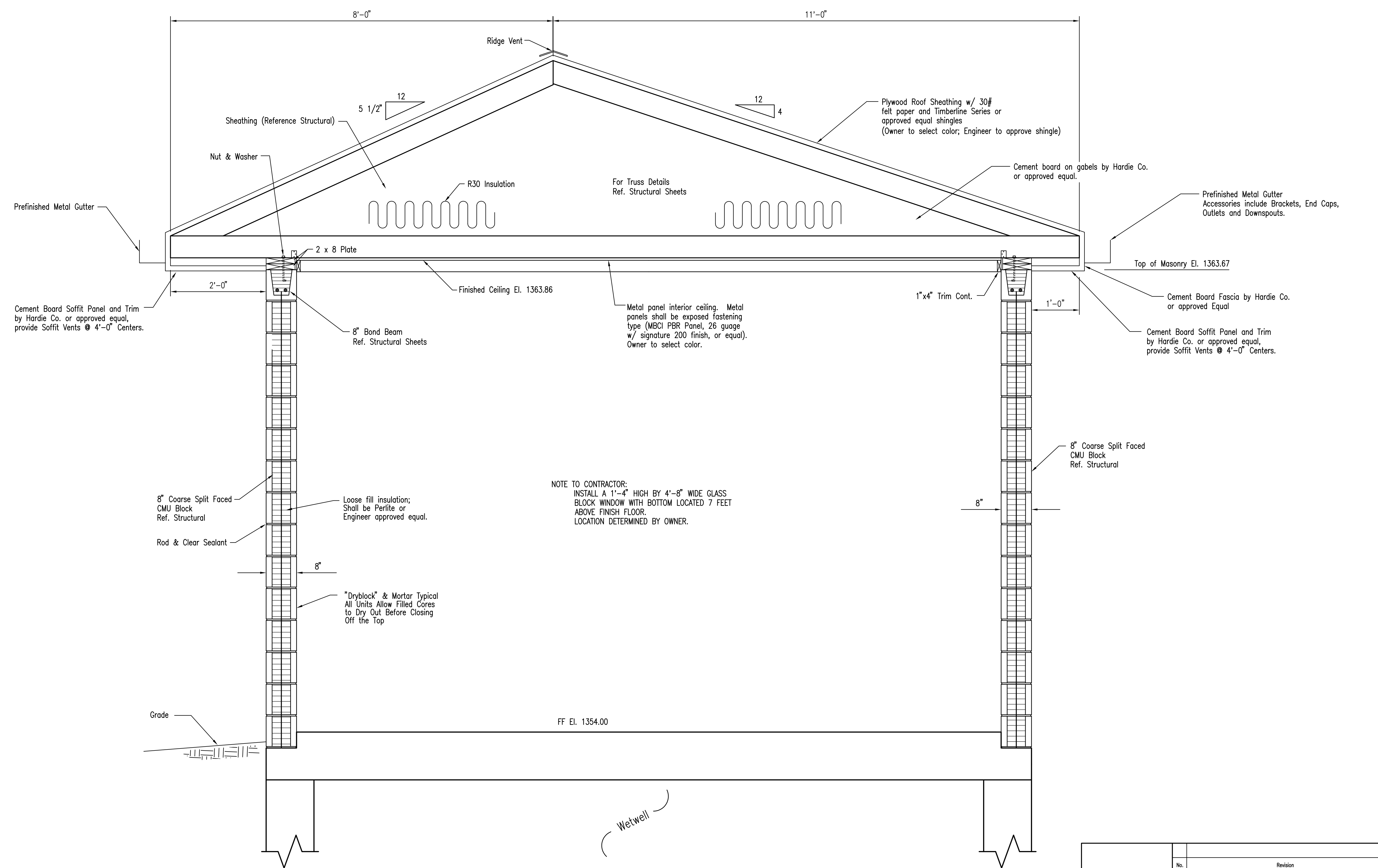
BUILDING SECTION SCALE: 1" = 1'-0"
