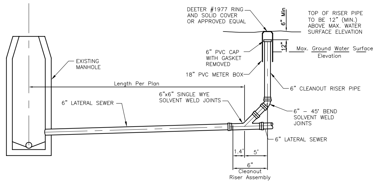
6" CLEANOUT RISER ASSEMBLY DETAIL
