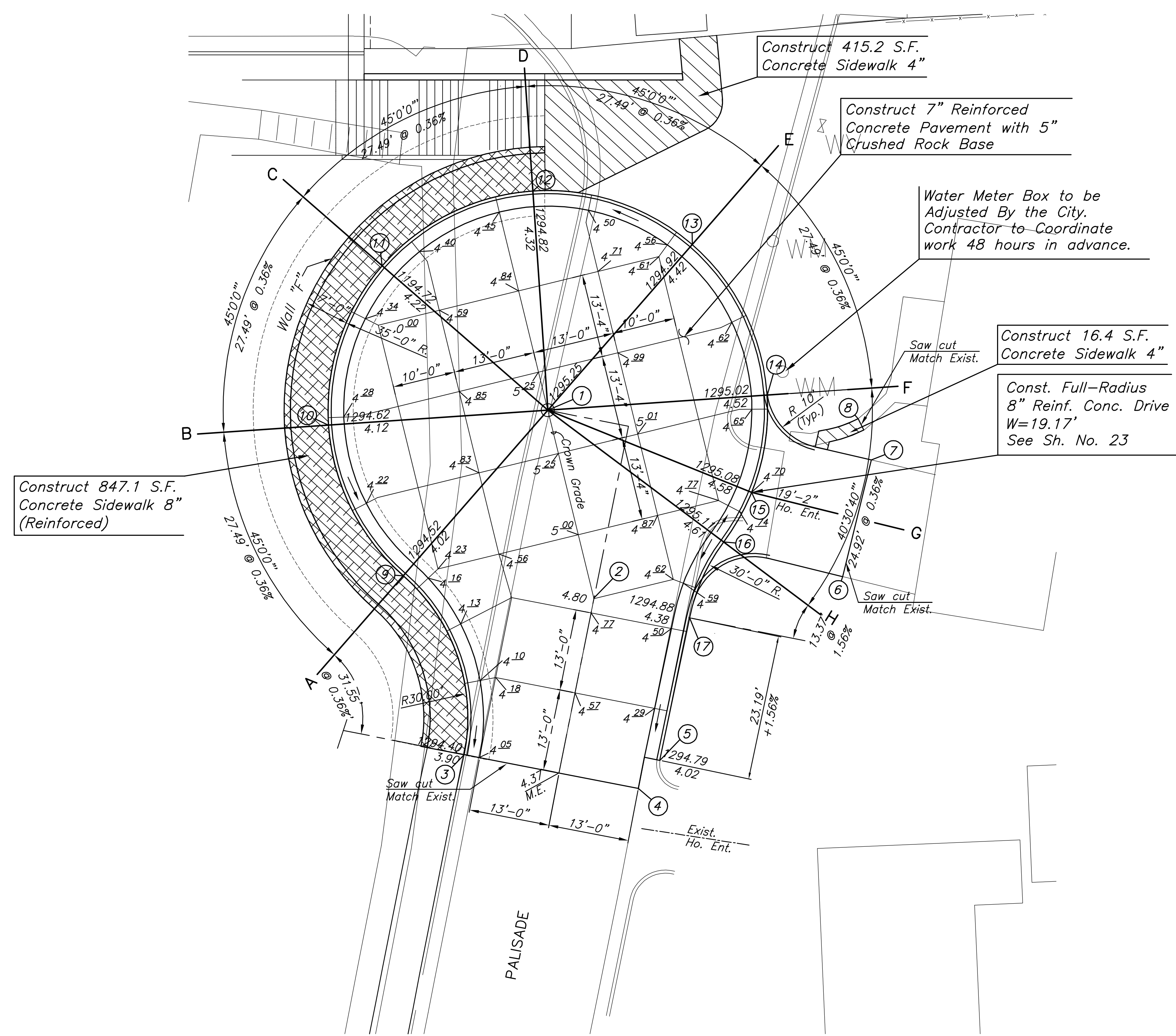
PALISADE STREET PAVING PLAN
