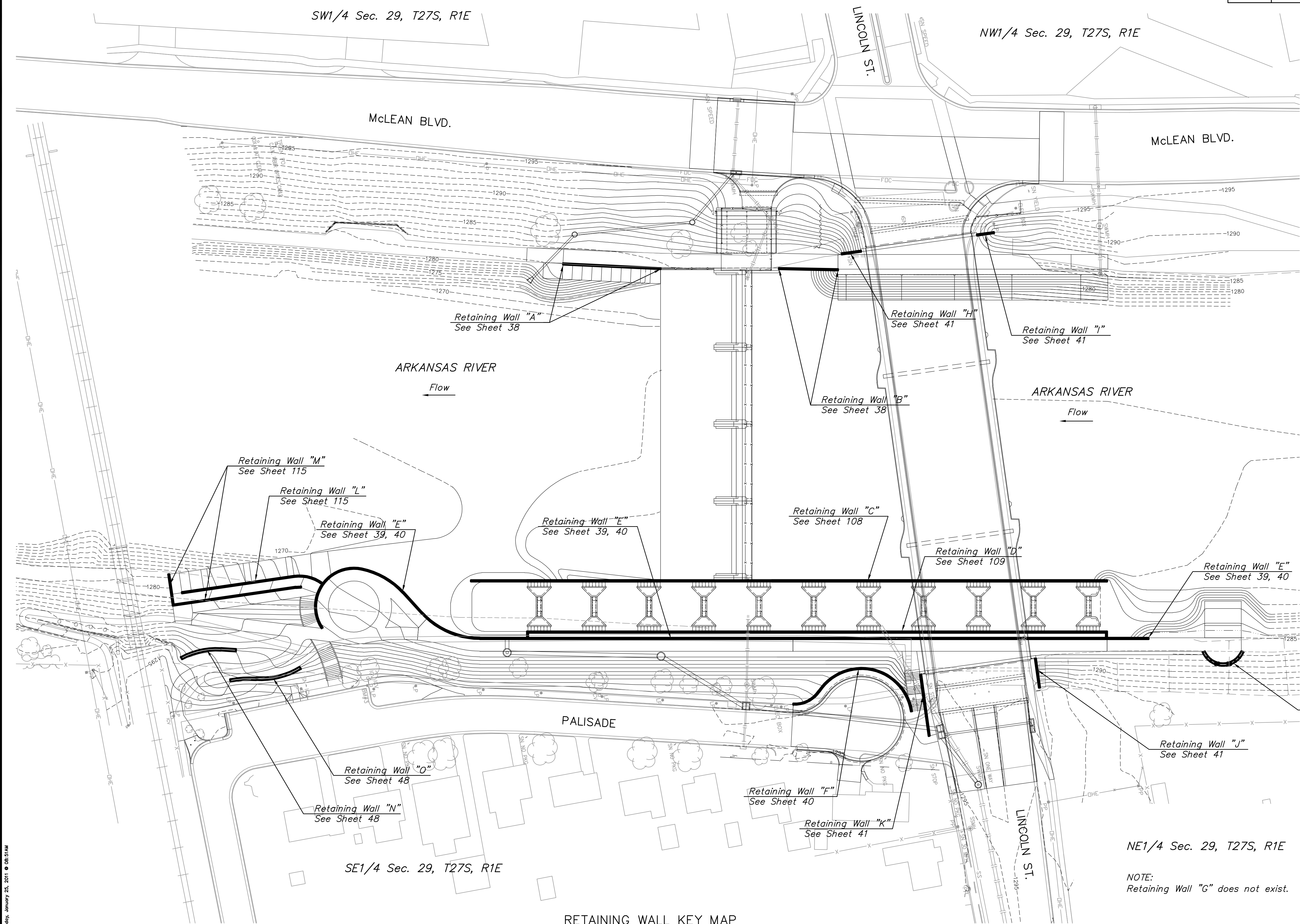
RETAINING WALL KEY MAP SCALE: 1"=40'
