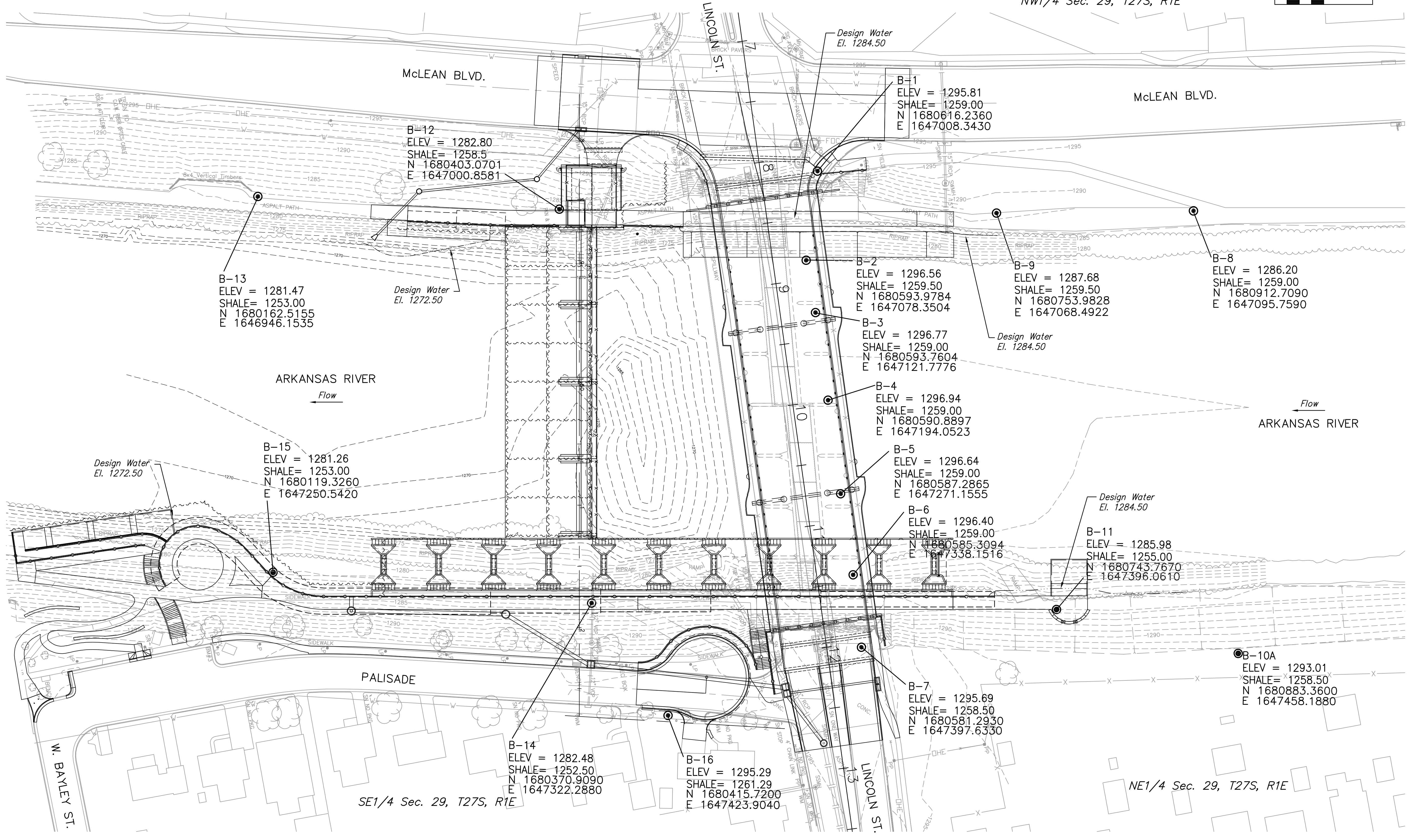
BORING LOCATION MAP SCALE: 1"=40'
