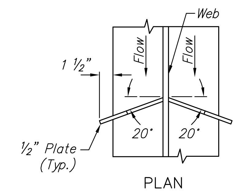
DRIP PLATE DETAIL Drip plates are located on the exterior beams as shown on framing plan
