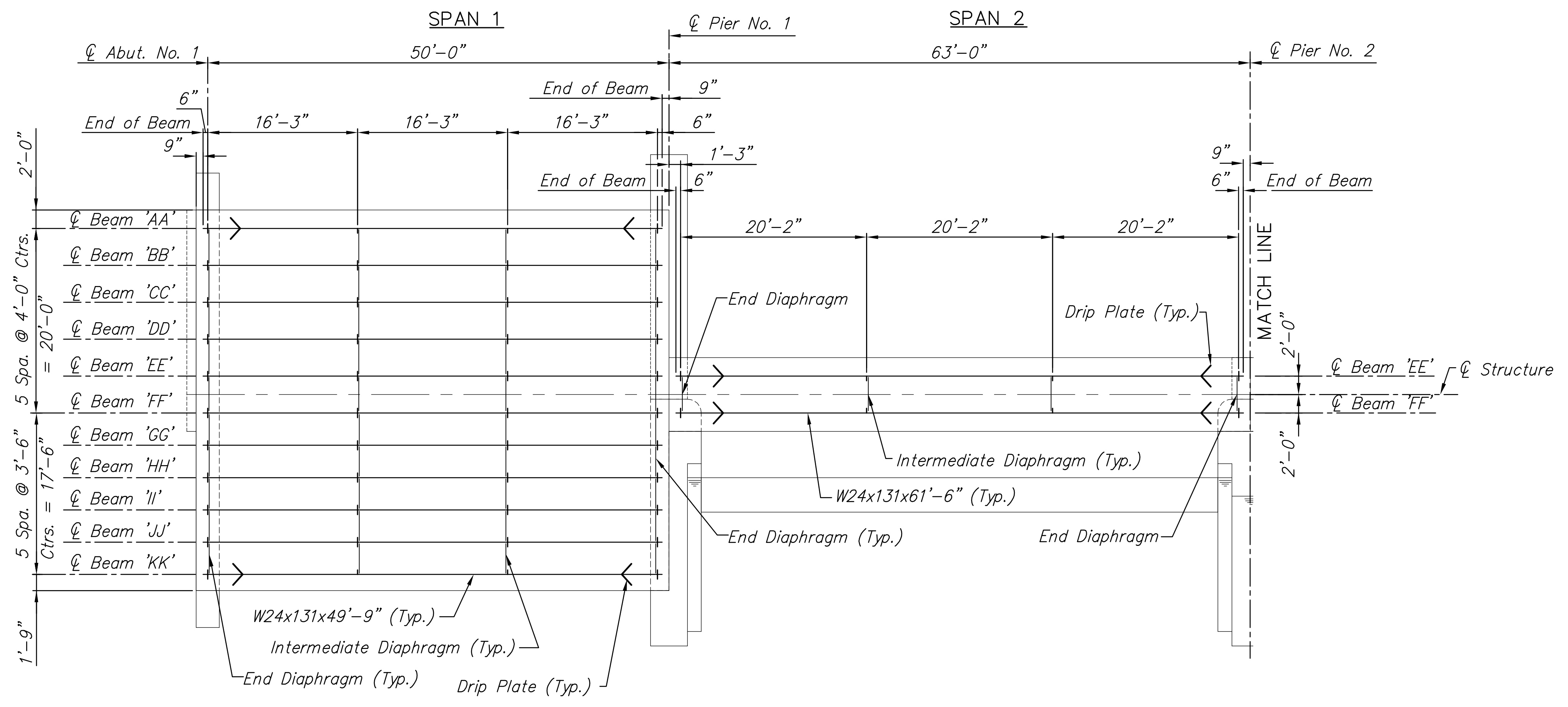
FRAMING PLAN - SPAN 1 & SPAN 2
