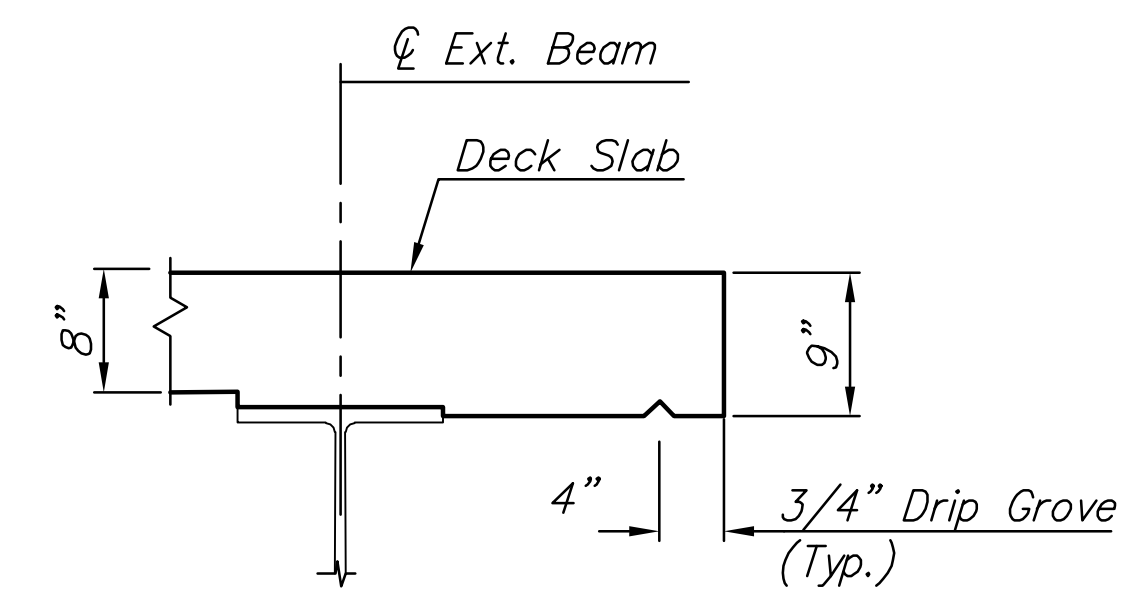
TYPICAL OVERHANG DETAILS
