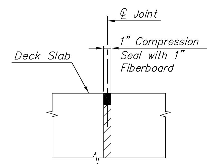
CONSTRUCTION JOINT AND COMPRESSION SEAL DETAIL
