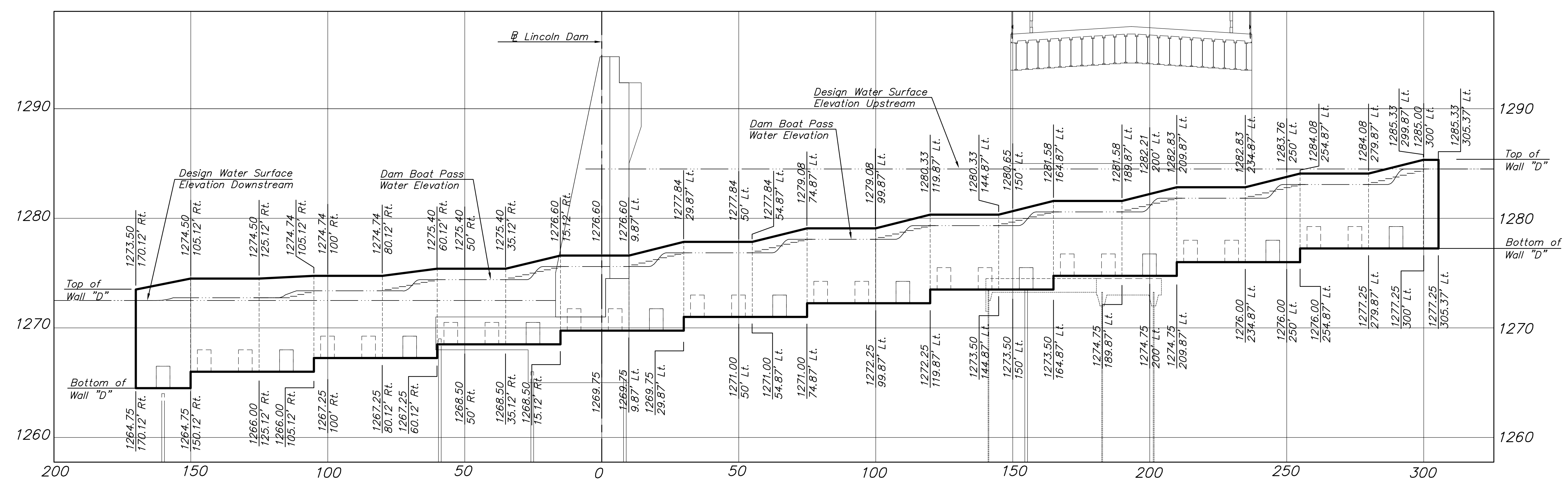
PROFILE OF BOAT/FISH PASS WALL "D"
