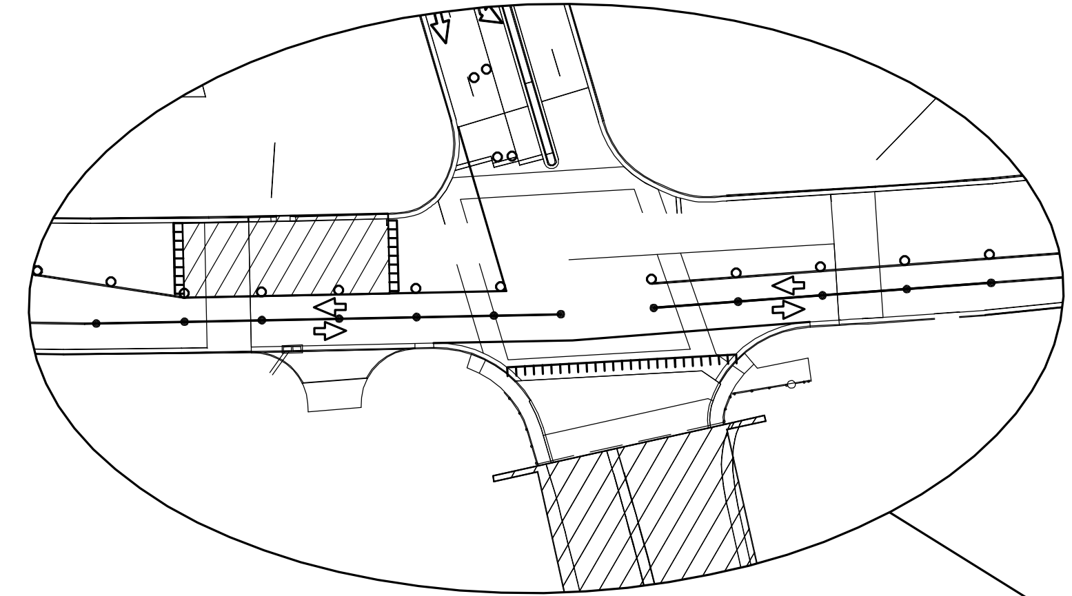
Insert: Utilize similar traffic control for construction of West lanes of McLean Blvd.
