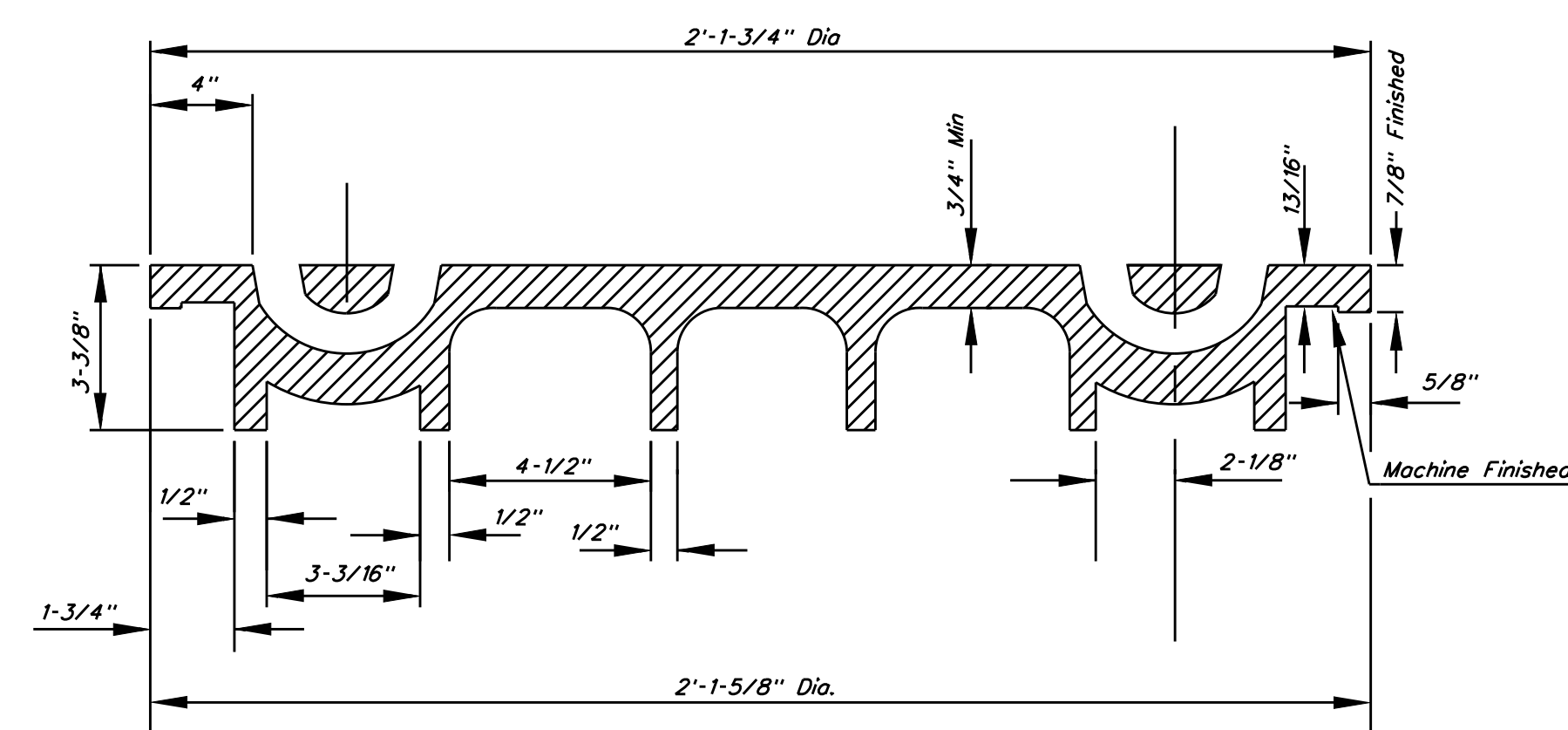
SECTION VIEW
