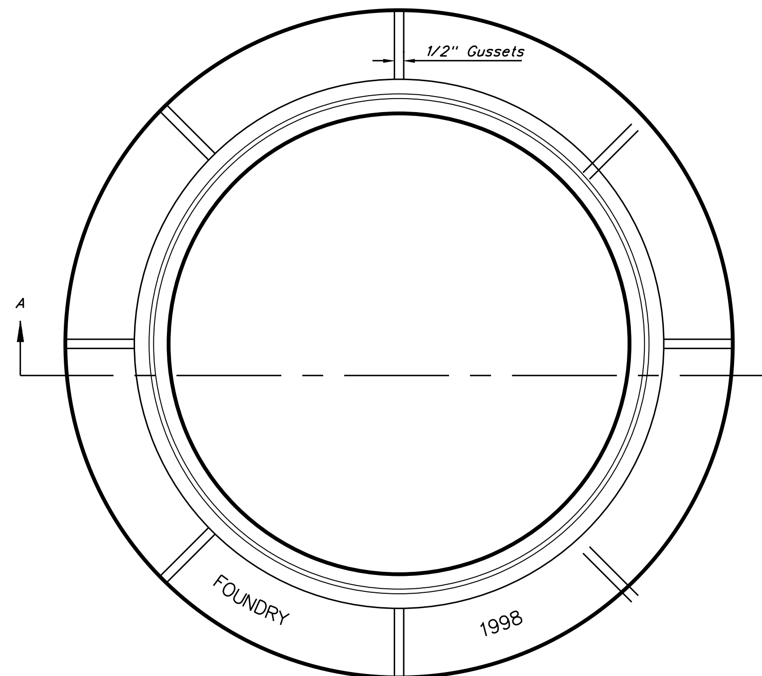
TOP VIEW
