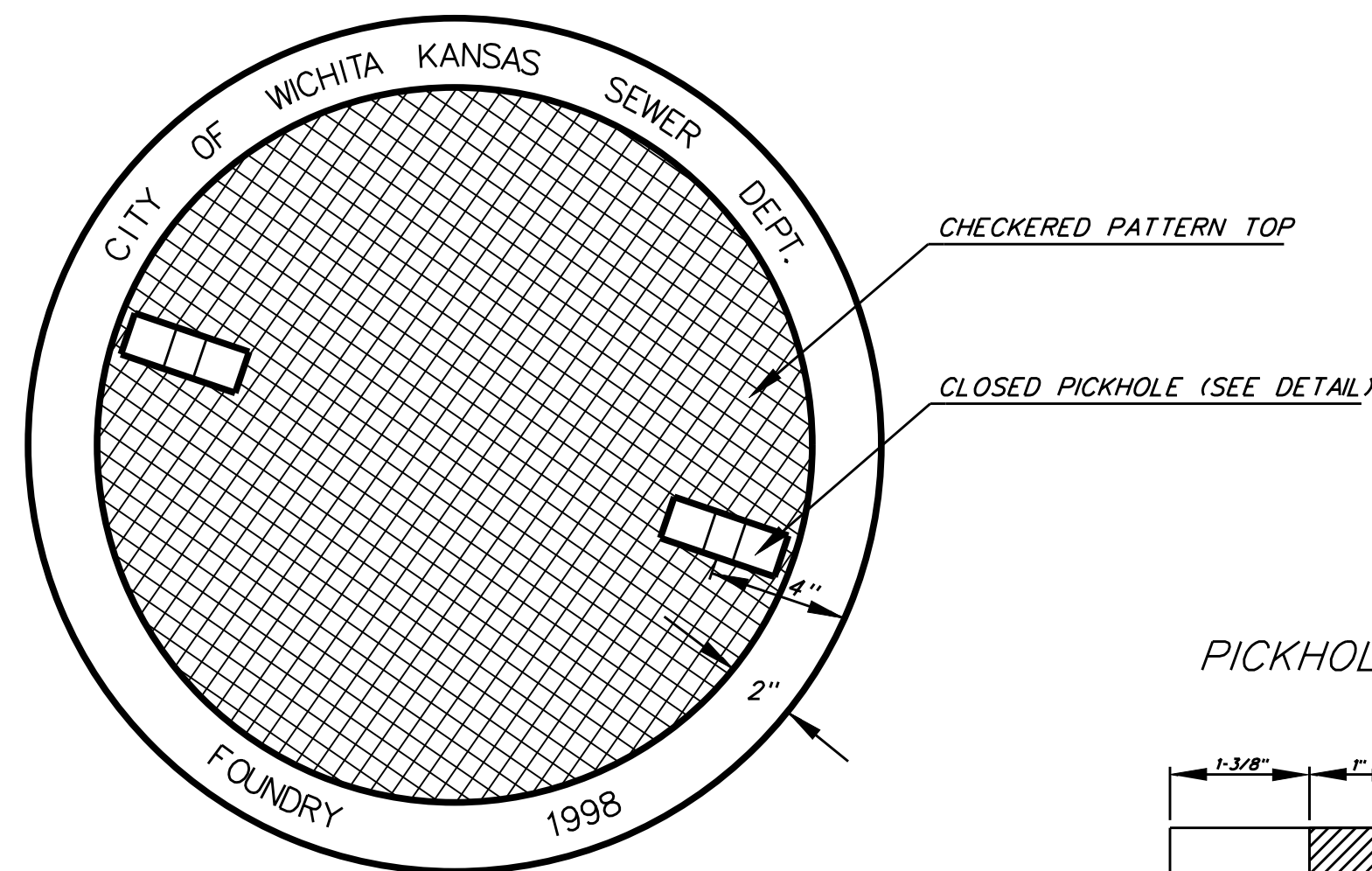
TOP VIEW
