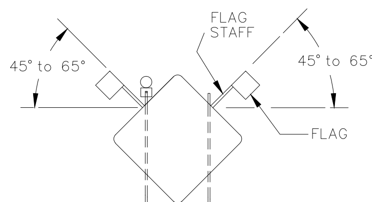
TYPE "A" LOW INTENSITY WARNING LIGHT MOUNTED TO SIGN POST
