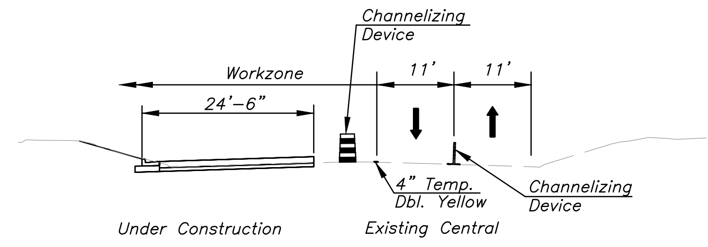
Phase I Traffic Control Section Looking East
