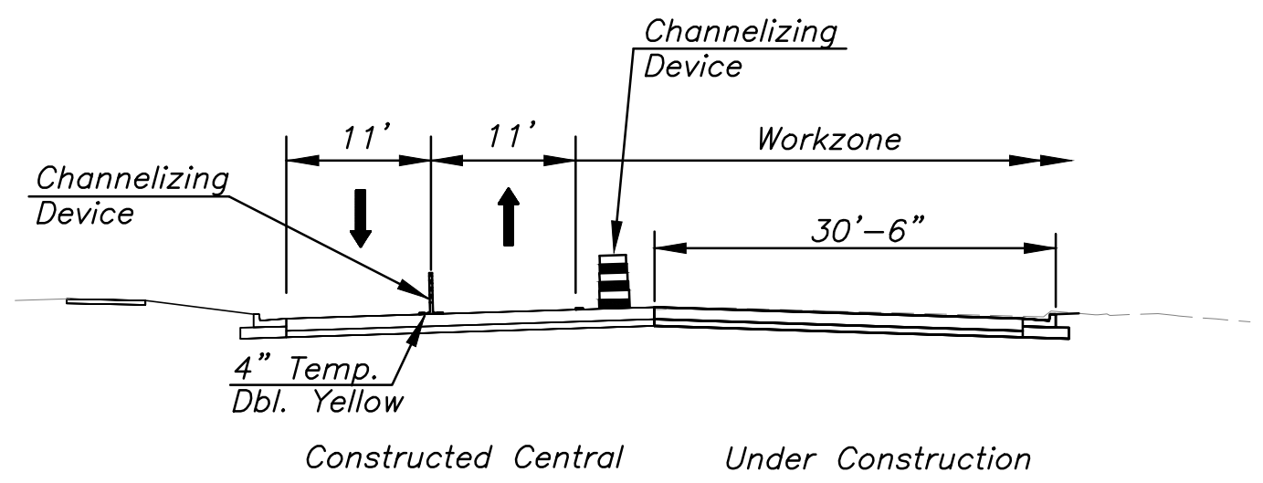
Phase 2 Traffic Control Section Looking East
