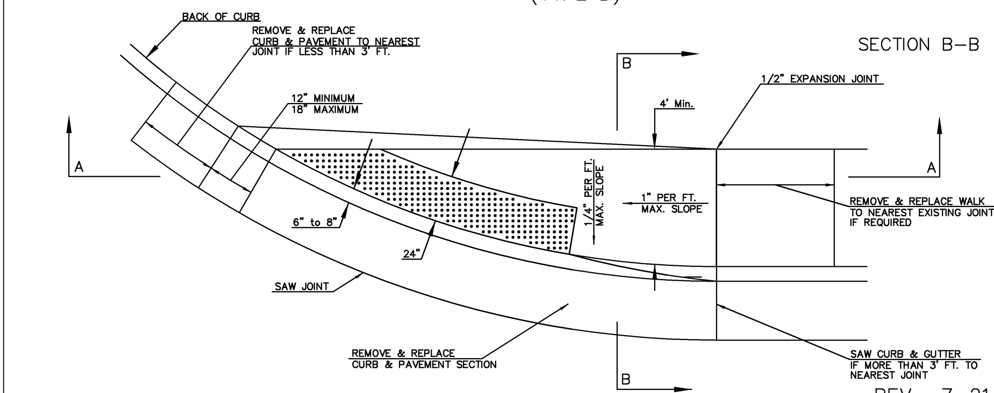
SECTION B-B
