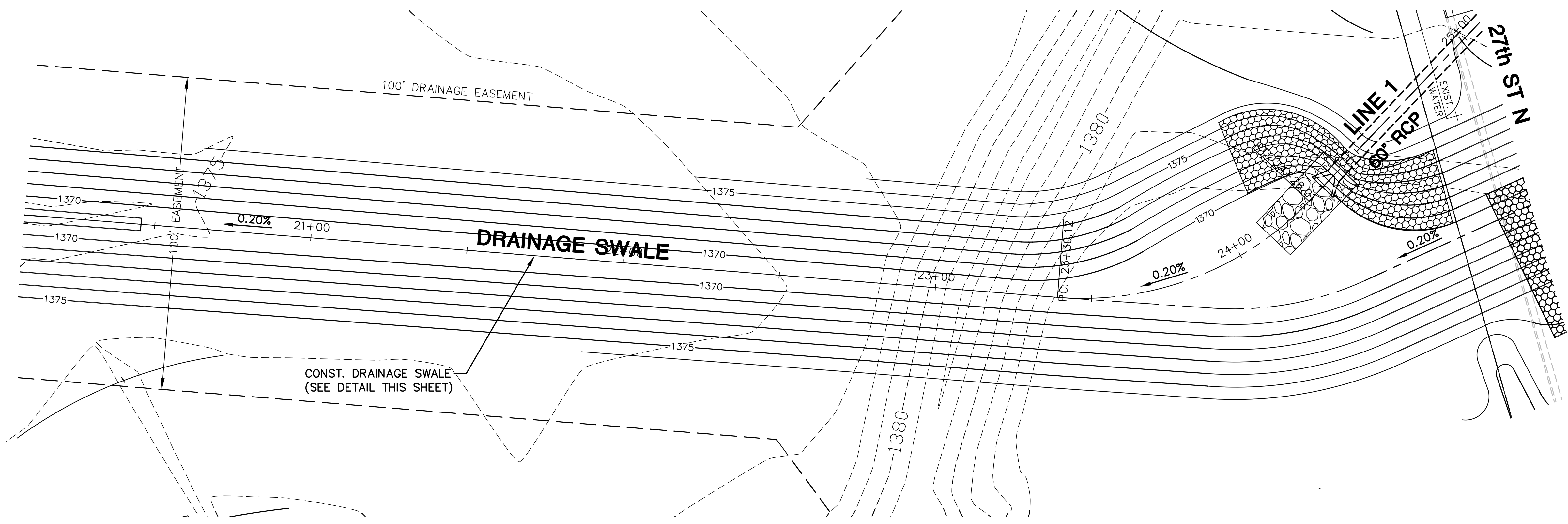
PLAN DRAINAGE SWALE PROFILE DRAINAGE SWALE
