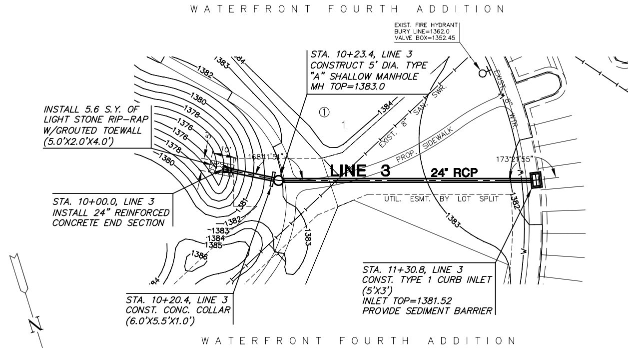
PLAN LINE 3 SCALE: 1"=20'
