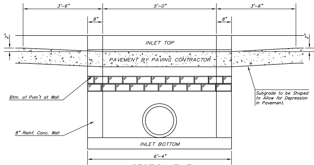
SECTION E-E
