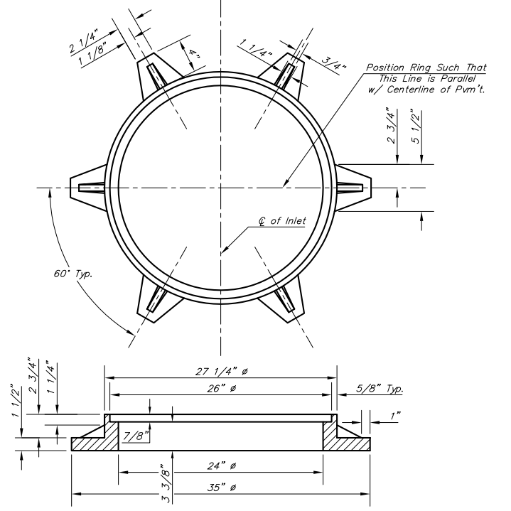
MANHOLE RING AND COVER
