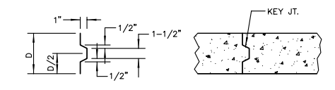
ALT. LONGITUDINAL CONSTRUCTION JOINT
