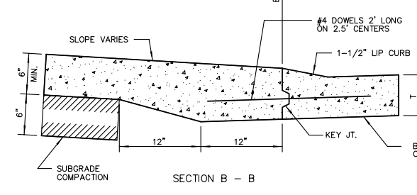
BACK OF CURB DETAIL
