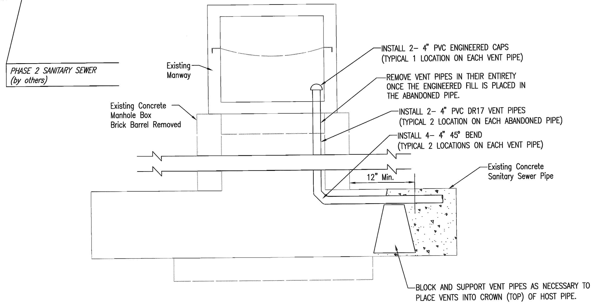
PLUG AND VENT PIPE DETAIL (NOT TO SCALE)
