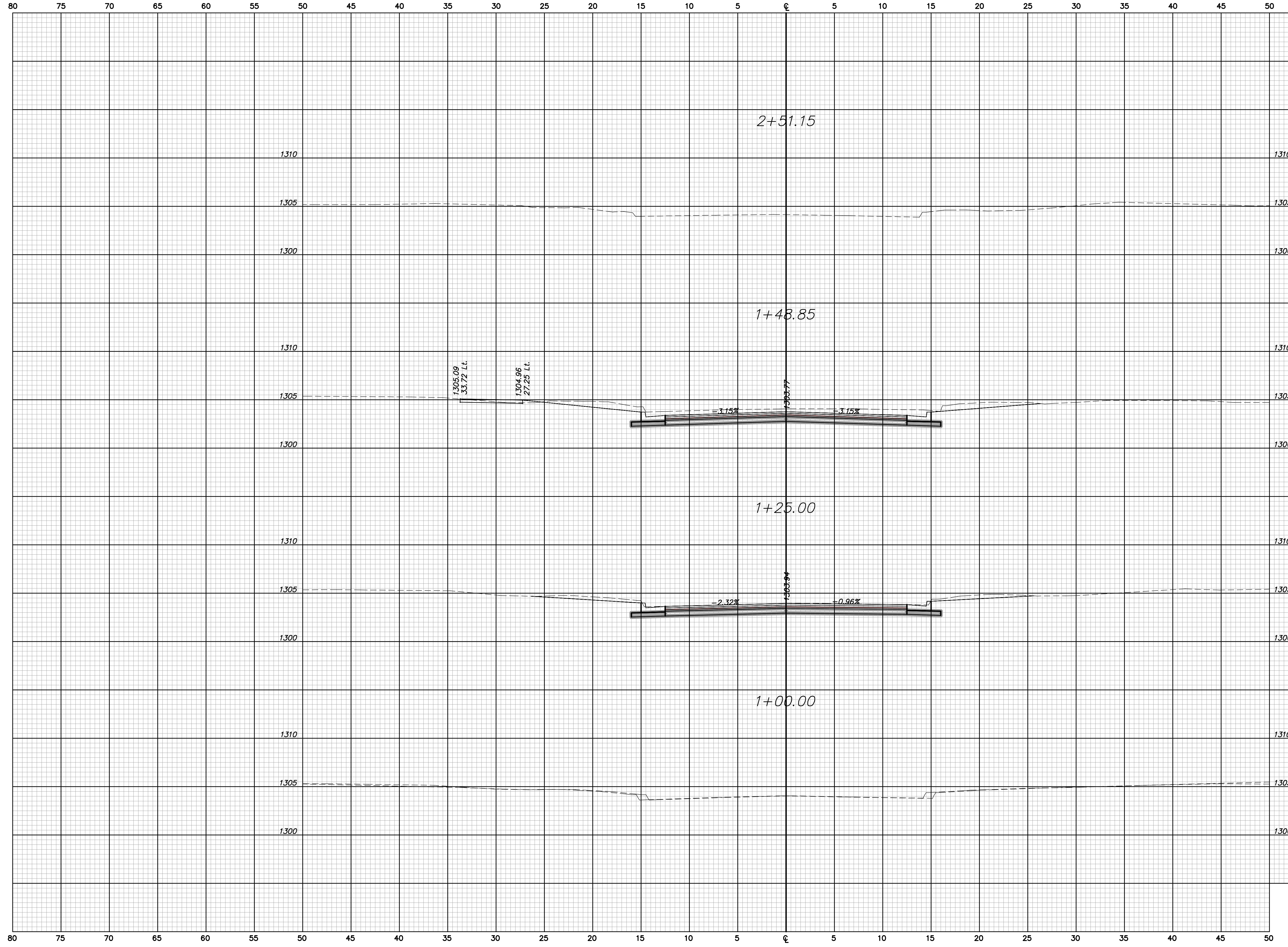
MADISON CROSS SECTIONS Sta. 1+00.00 to Sta. 2+51.15
