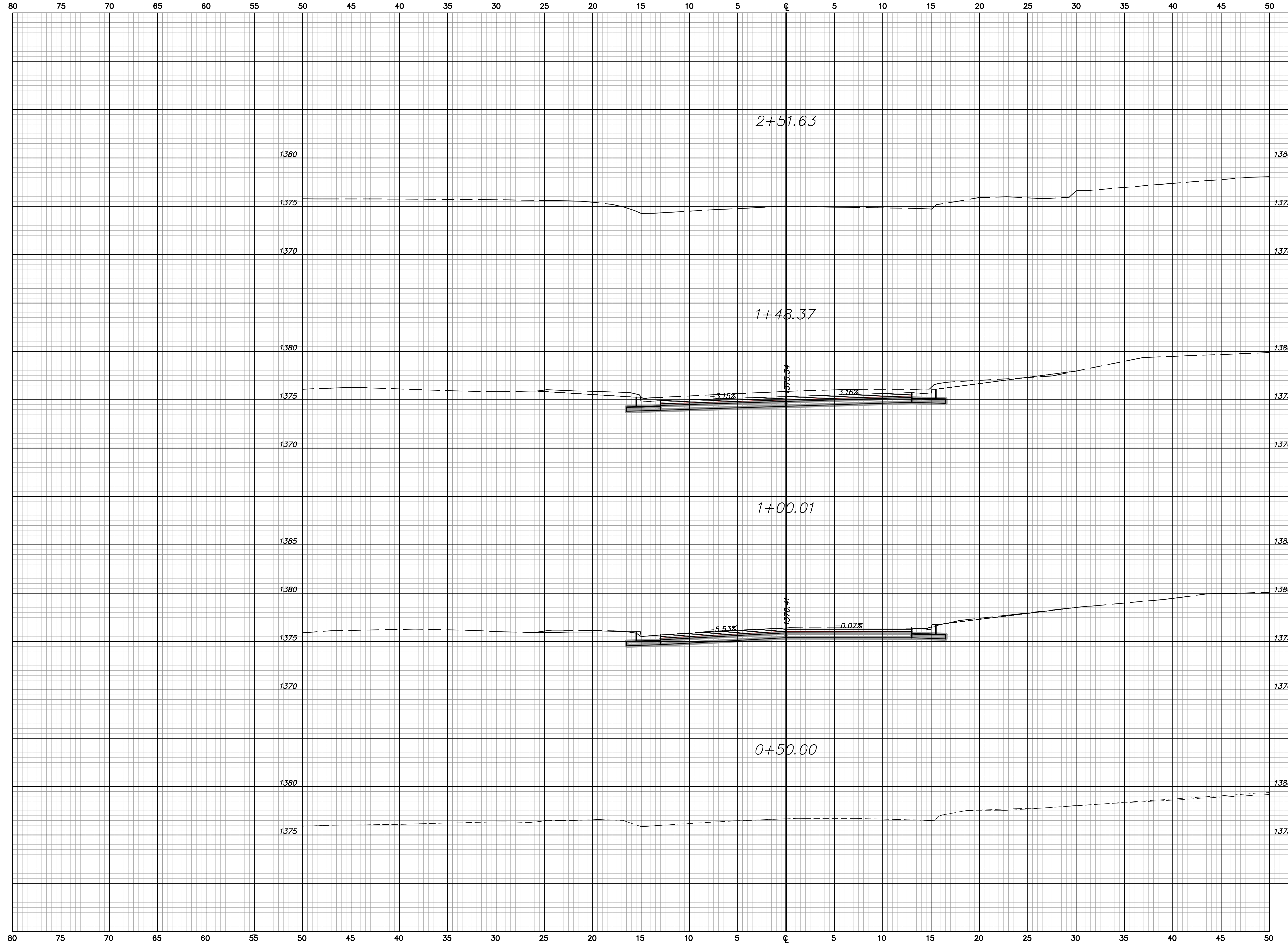
VASSAR CROSS SECTIONS Sta. 0+50.00 to Sta. 2+51.63
