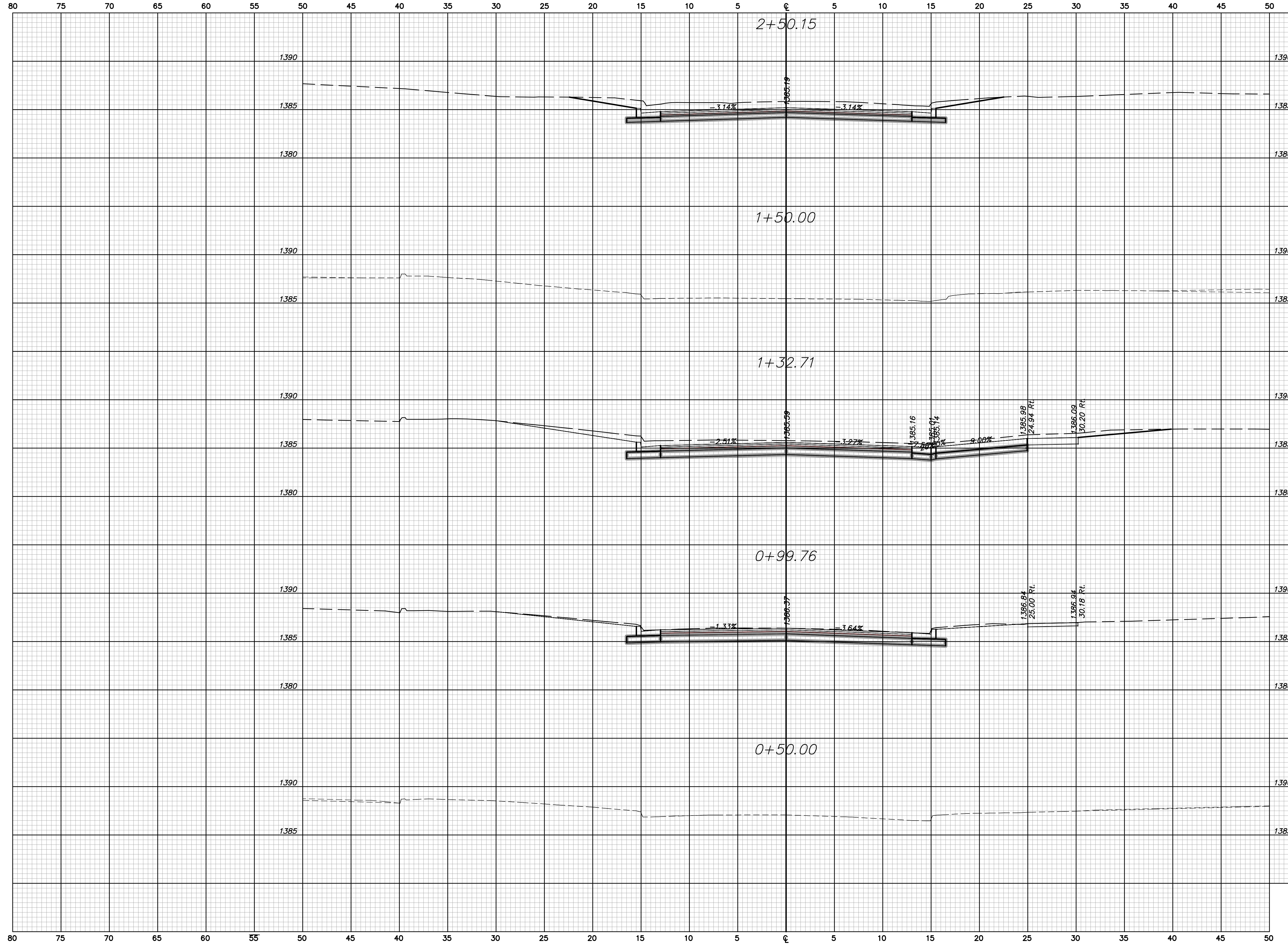
TERRACE CROSS SECTIONS Sta. 0+50.00 to Sta. 2+50.15
