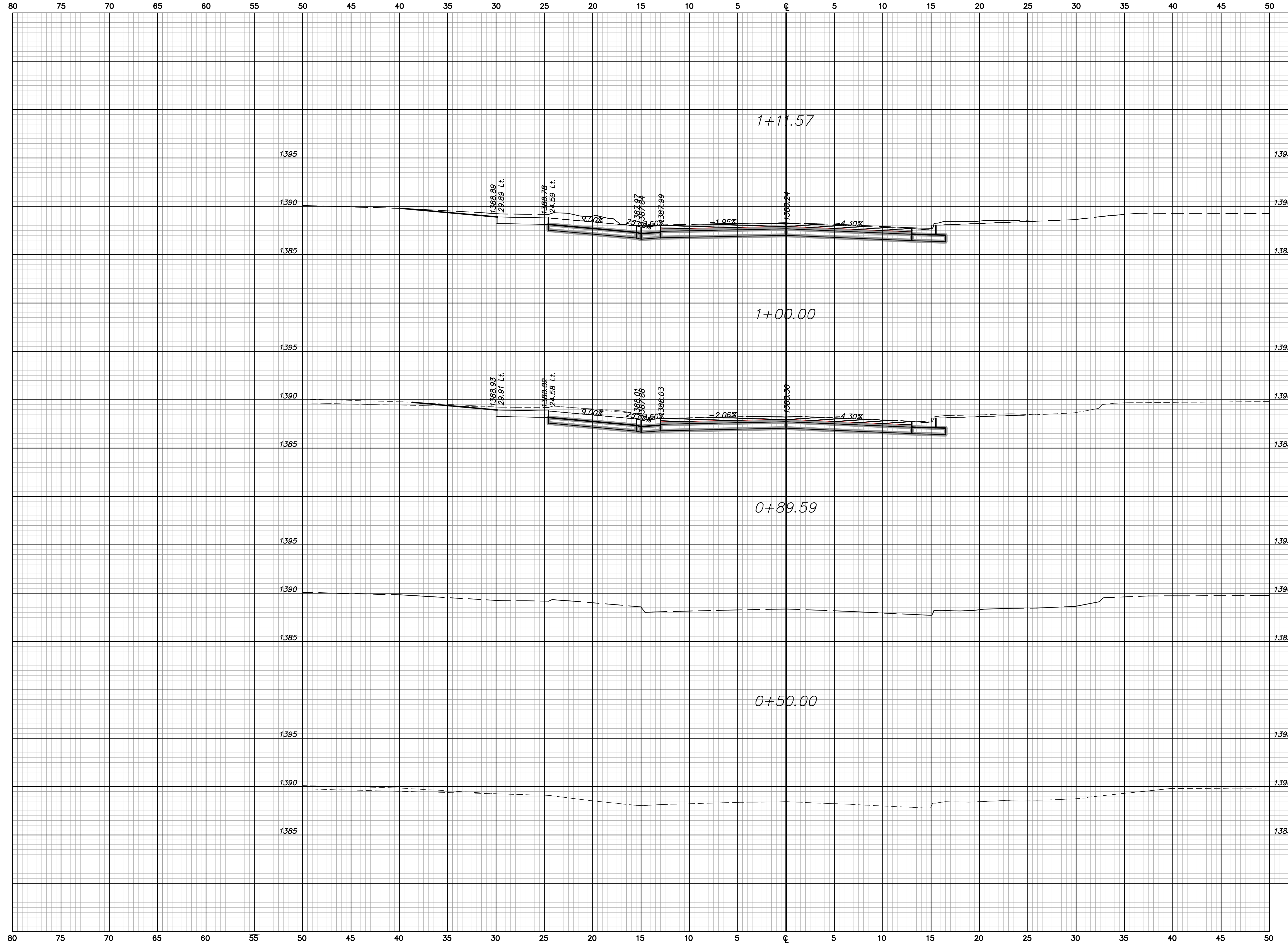
PERSHING CROSS SECTIONS Sta. 0+50.00 to Sta. 1+26.23
