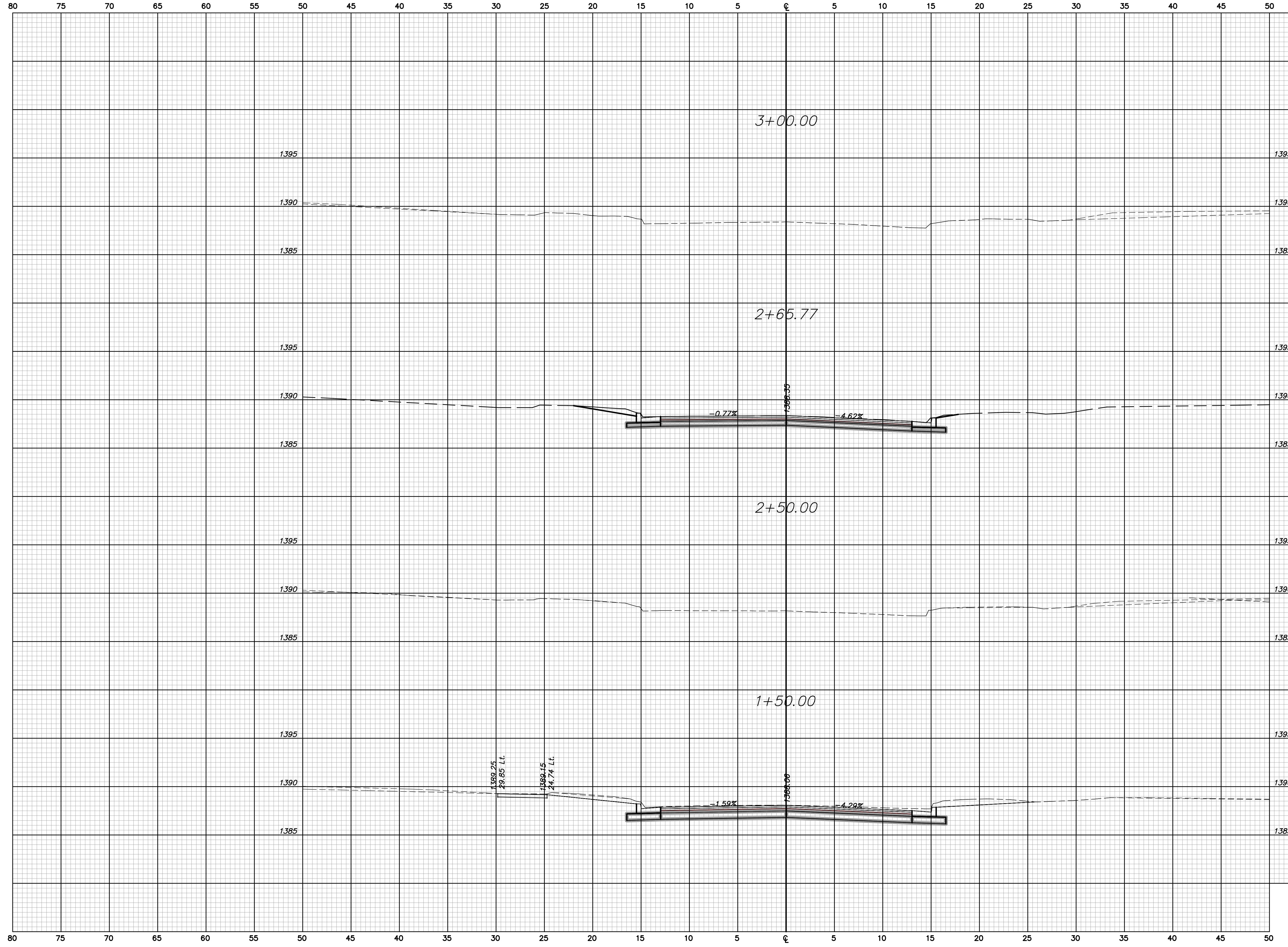
PERSHING CROSS SECTIONS Sta. 1+50.00 to Sta. 3+00.00
