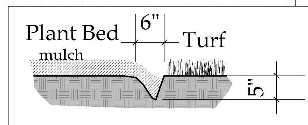
1 Trenched "V" Plant Bed Edge 1" = 1'-0"
