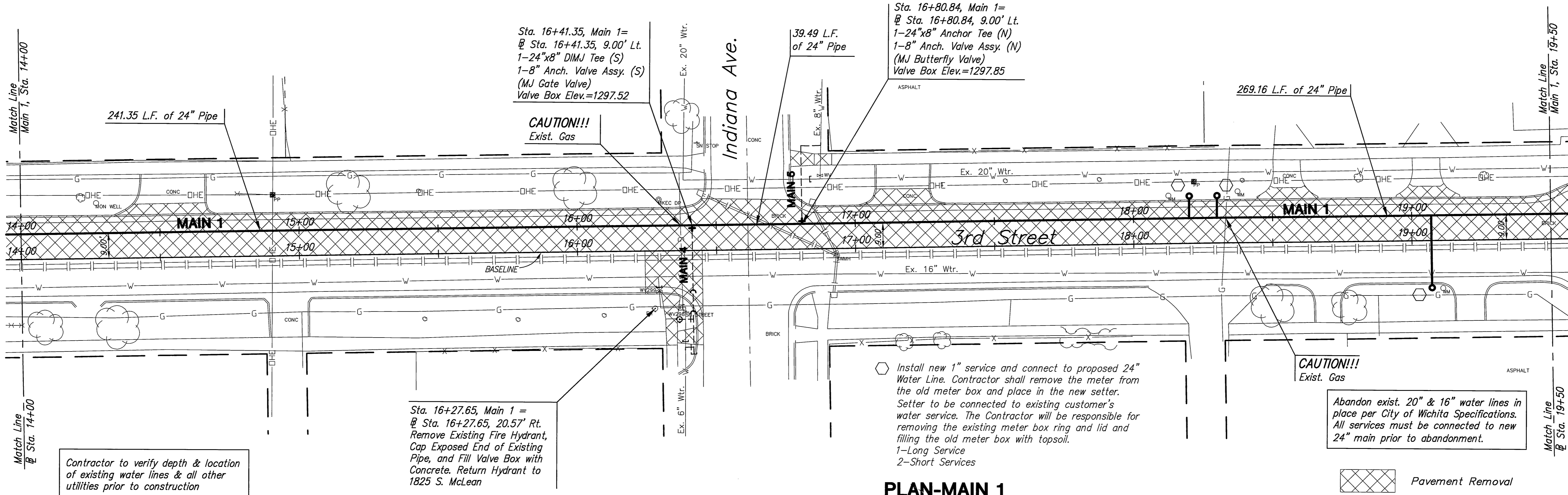
PLAN-MAIN 1 SCALE: 1"=20'
