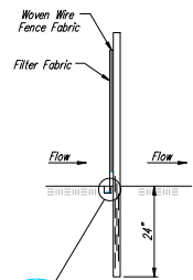
ANCHOR TRENCH DETAIL
