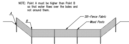
SILT FENCE DITCH CHECKS (STREAM PROTECTION)
