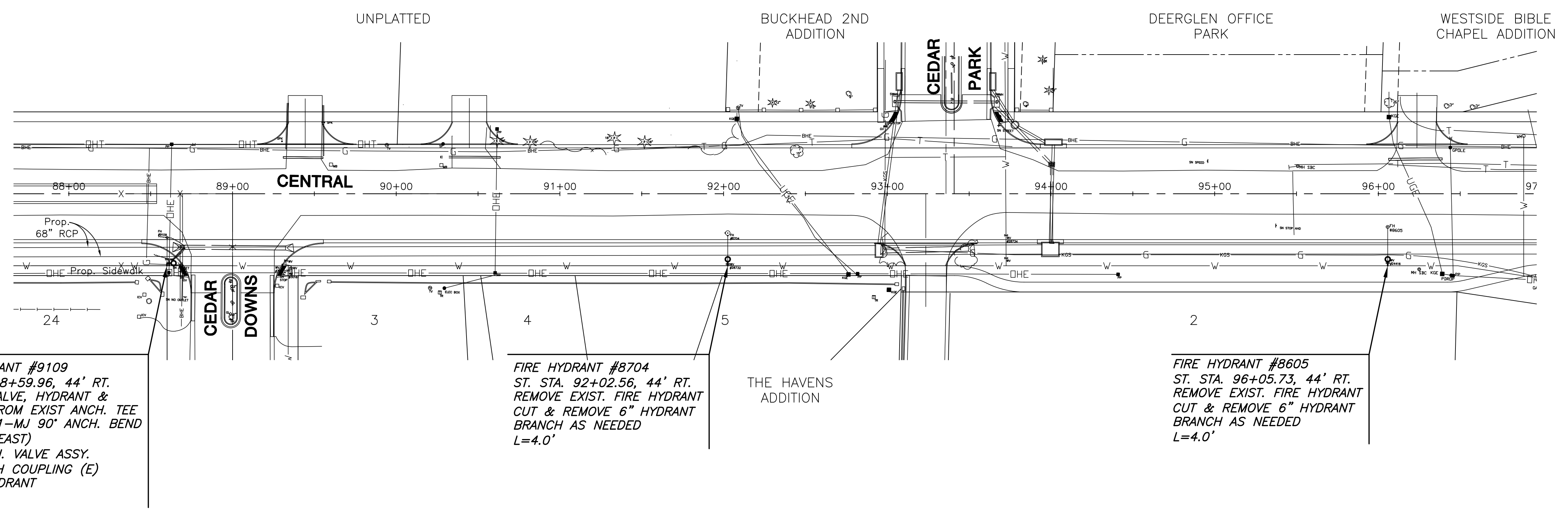
PLAN FIRE HYDRANT 9109
