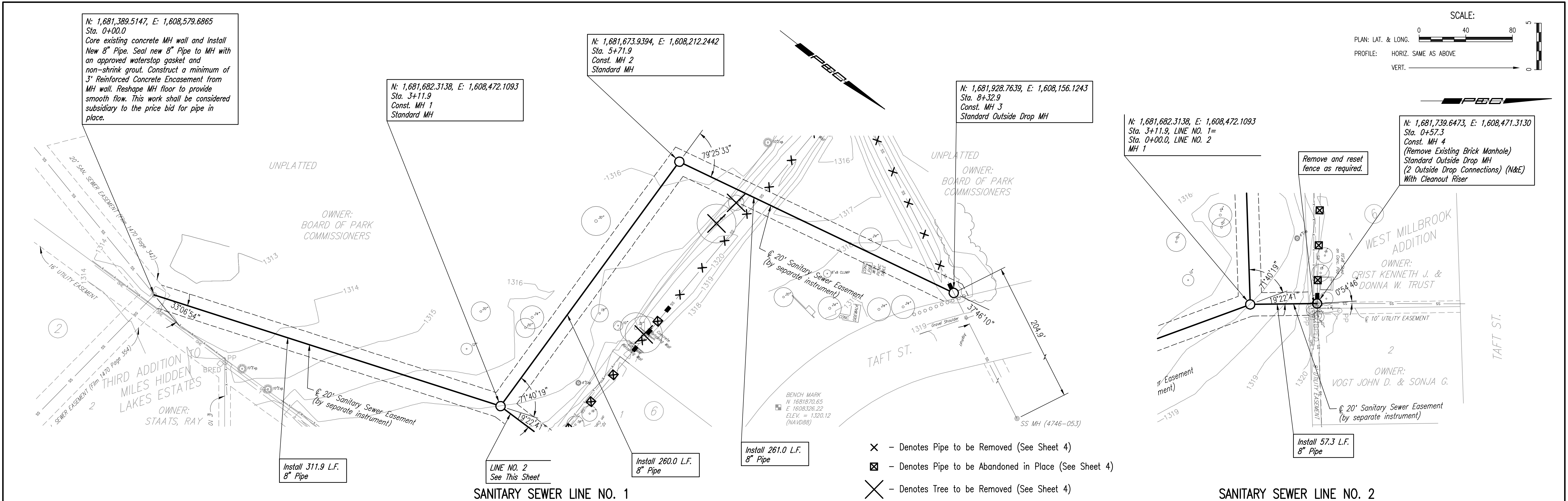
SANITARY SEWER LINE NO. 1
