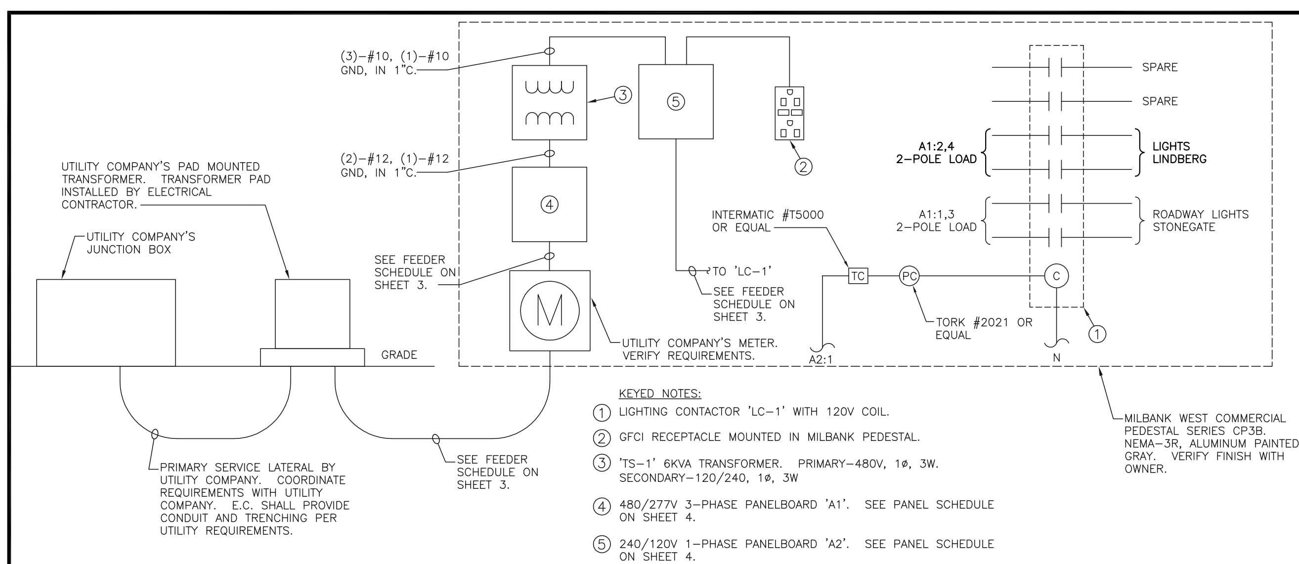
4 WIRING DIAGRAM FOR EXISTING ELECTRICAL PEDESTAL 'A' NO SCALE
