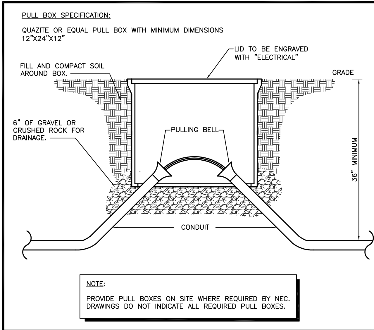
2 PULL BOX DETAIL NO SCALE
