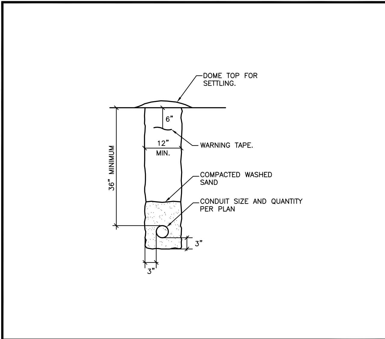
3 TYPICAL TRENCH TRENCH CROSS SECTION NO SCALE
