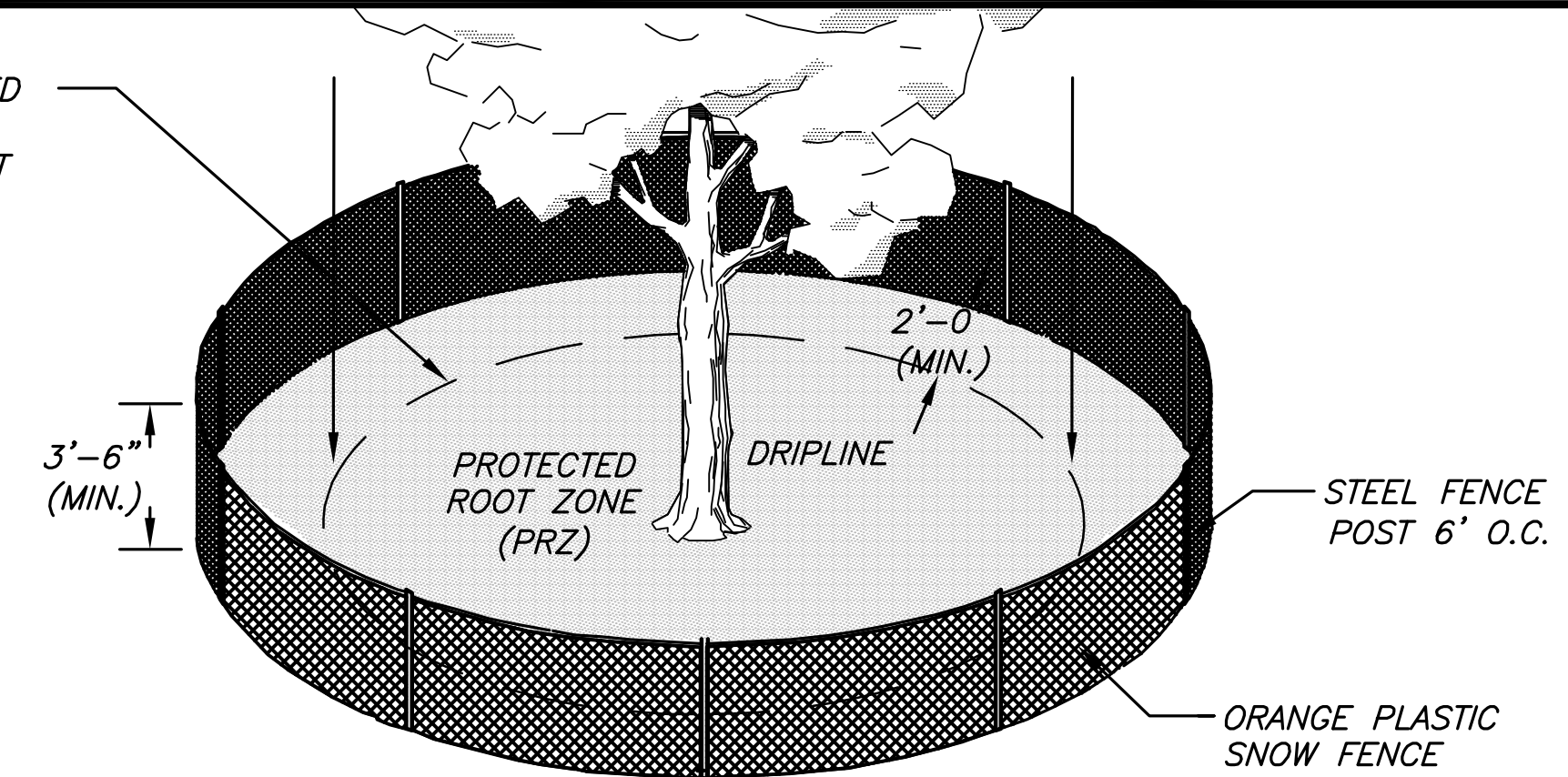
TEMPORARY TREE PROTECTION NOT TO SCALE
