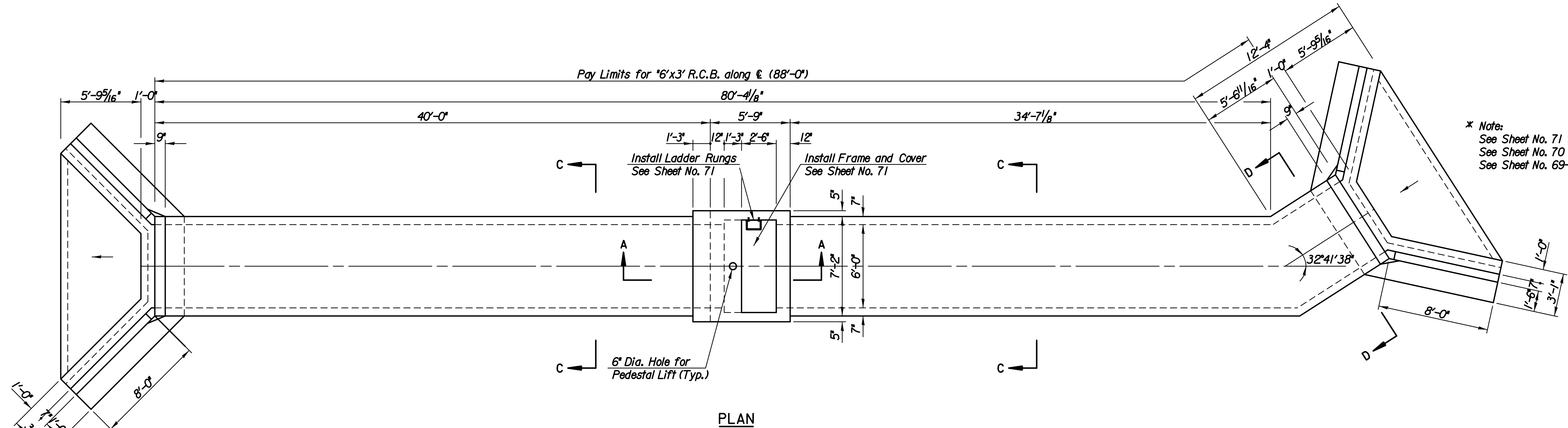
PLAN
