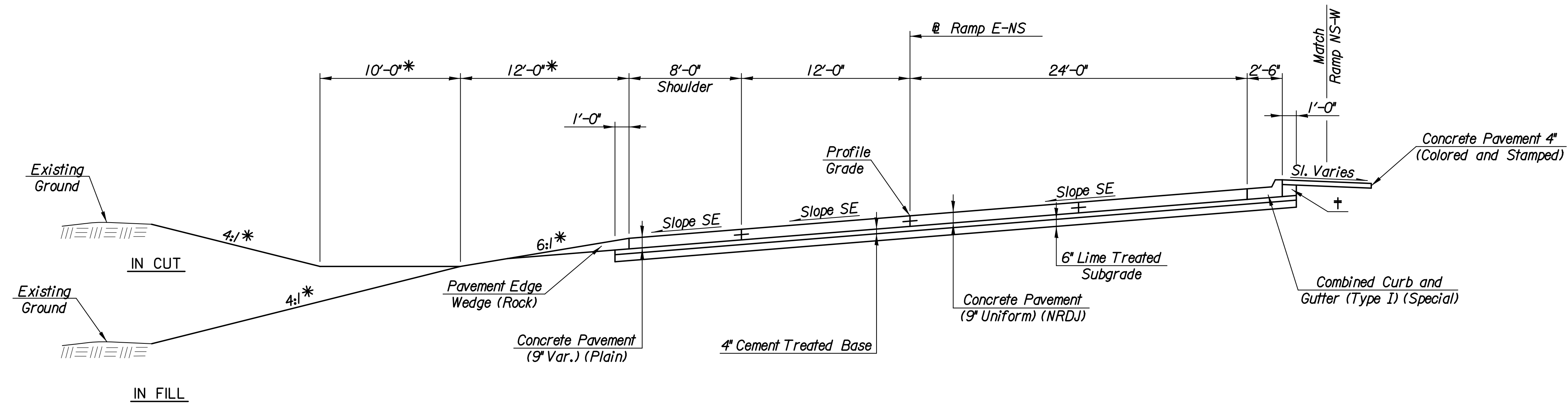
TYPICAL SECTION Sta. 452+48.49 to Sta. 454+85.13
