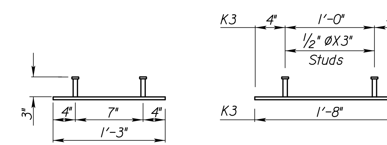
ELEV. OF BRG. PLATE TYPICAL SECTION
