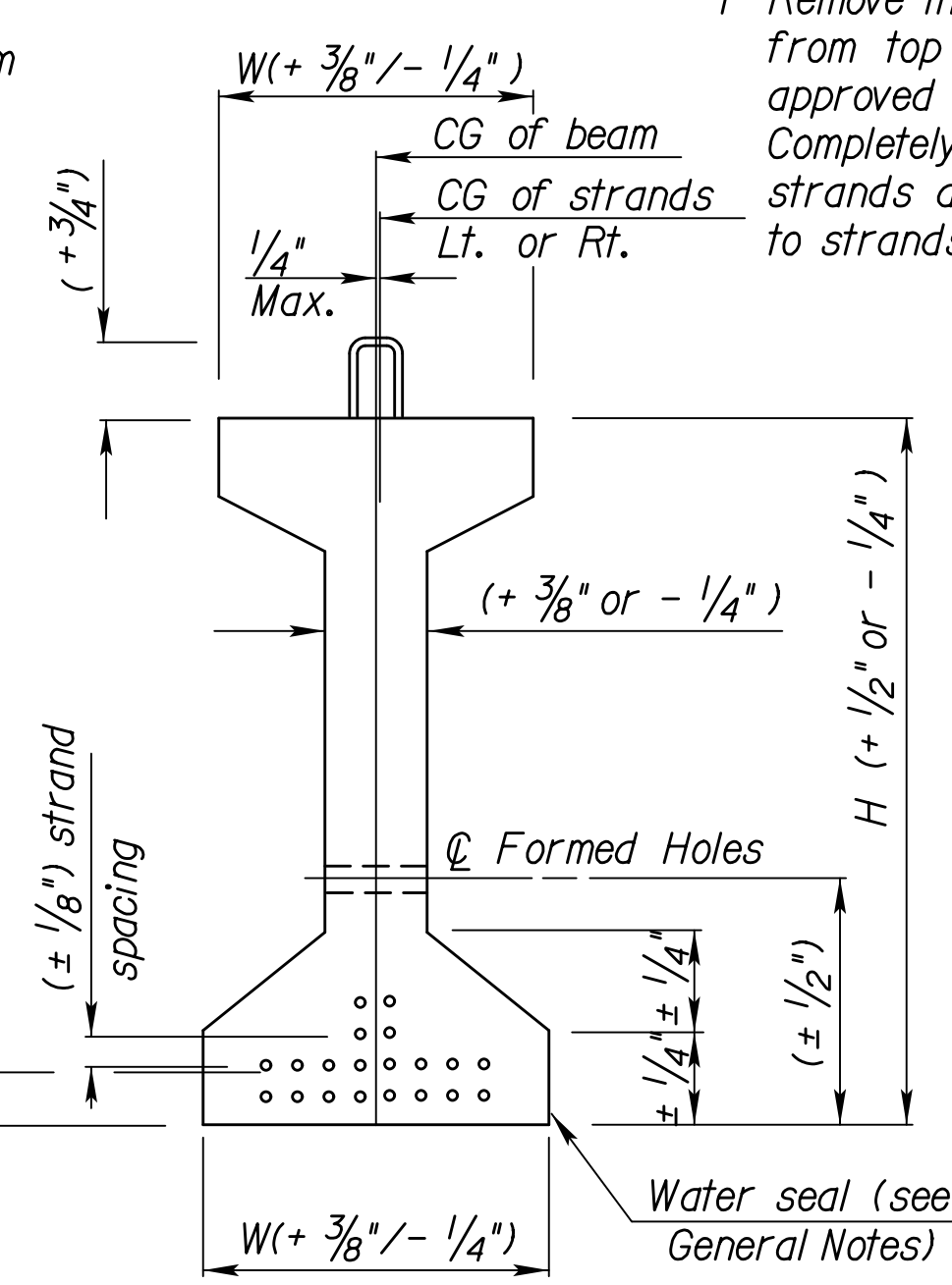
TYPICAL SECTION
