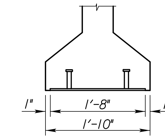
END VIEW (K3 Beam)
