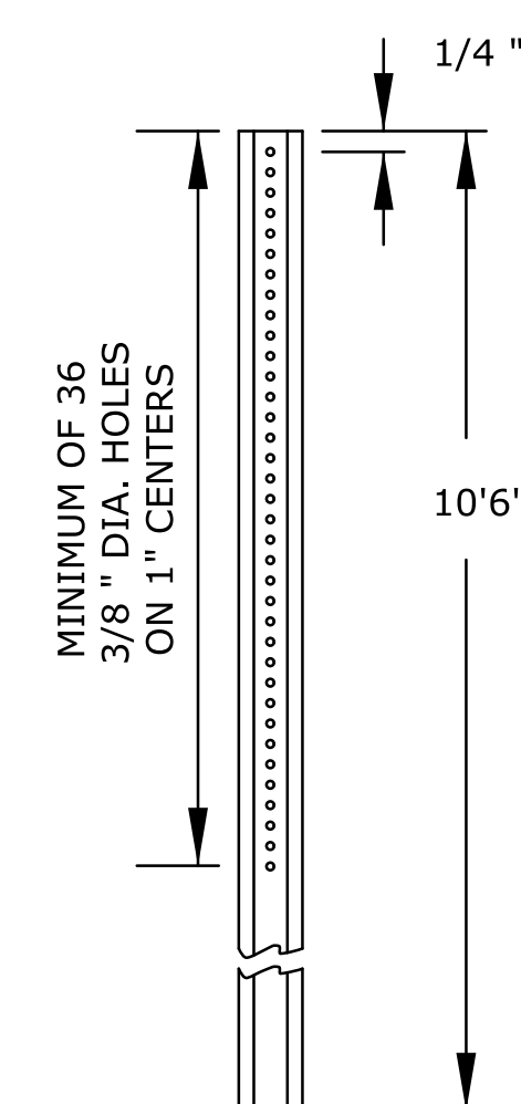
'U' POST PUNCHING DETAILS
