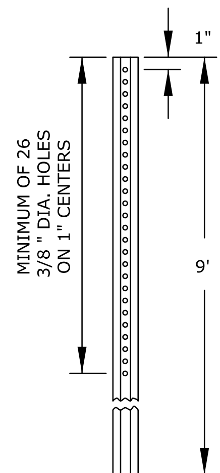
PUNCHING DETAILS
