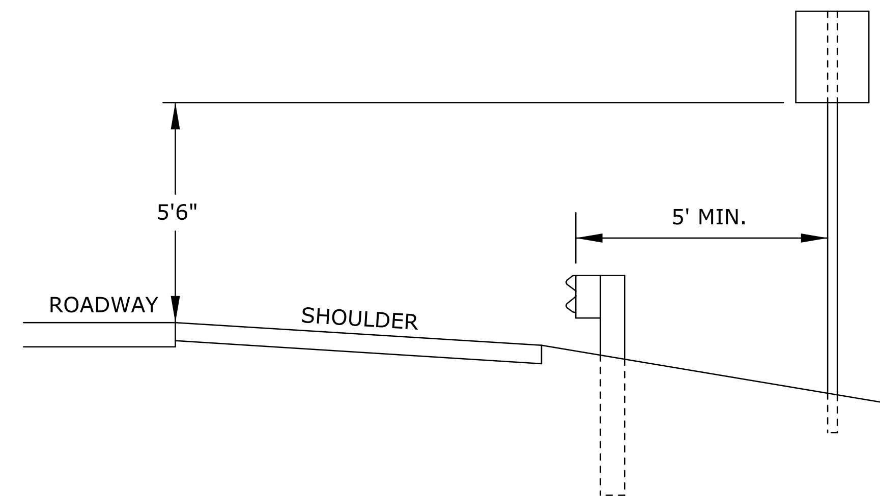
GUARD FENCE SECTION
