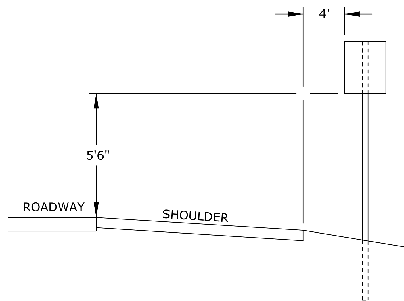
SHOULDER SECTION
