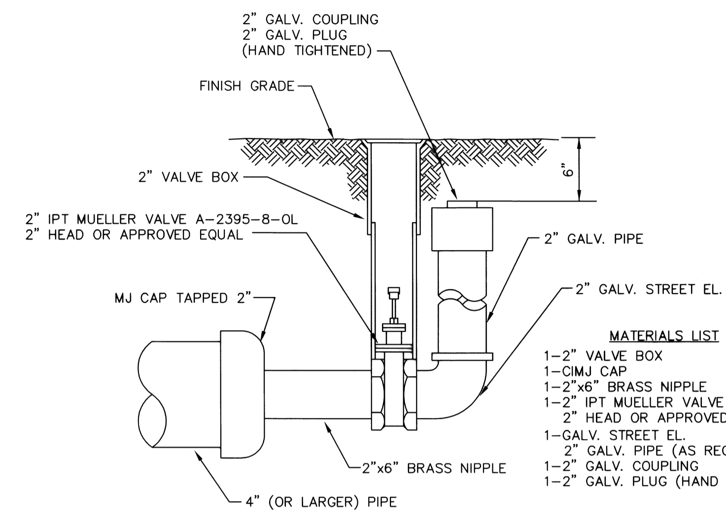
2" BLOWOFF ASSEMBLY
