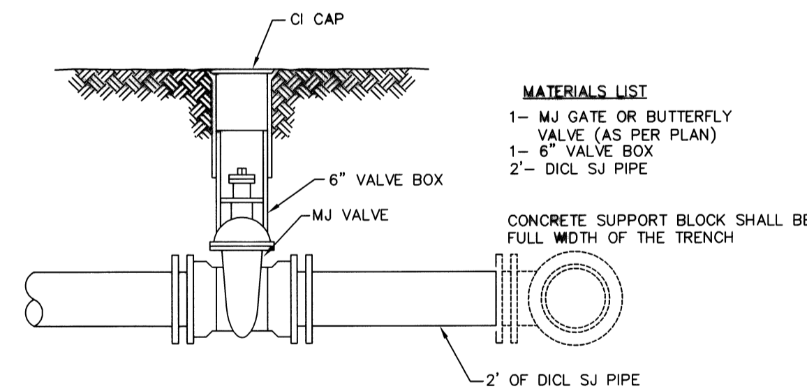
VALVE ASSEMBLY
