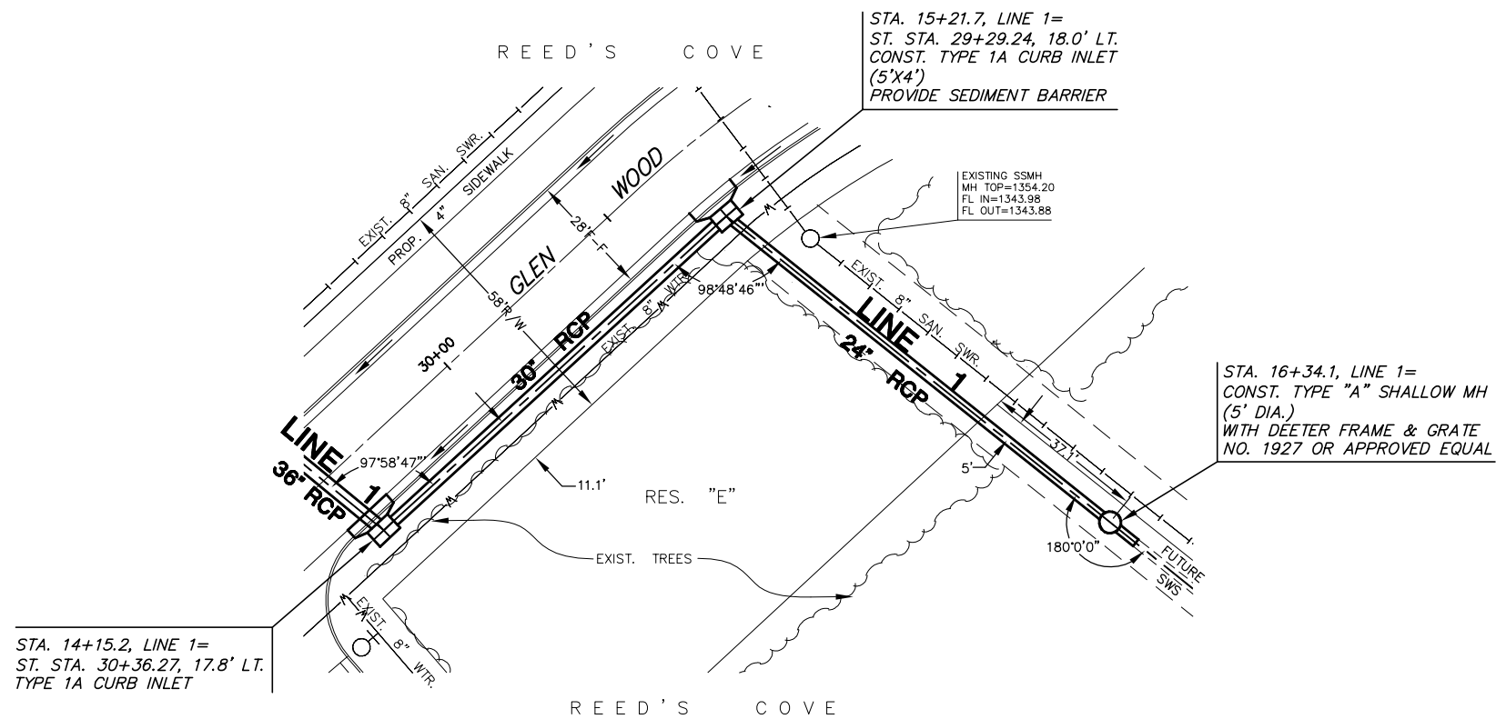
PLAN LINE 1
