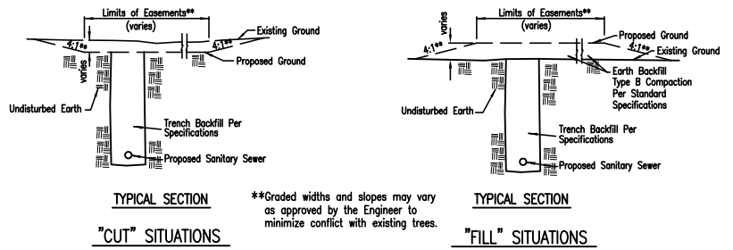
EASEMENT GRADING DETAILS
