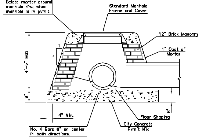
SPECIAL SHALLOW TYPE "B" MANHOLE
