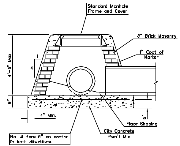
SPECIAL SHALLOW TYPE "A" MANHOLE
