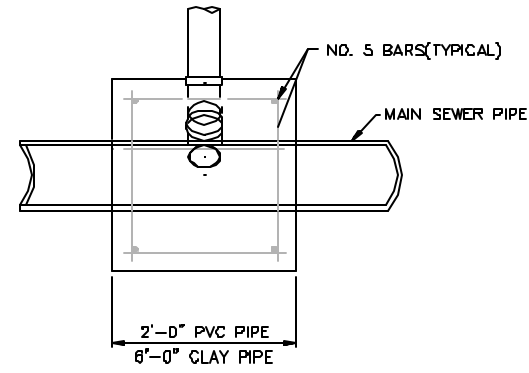
TYPICAL SECTION X-X
