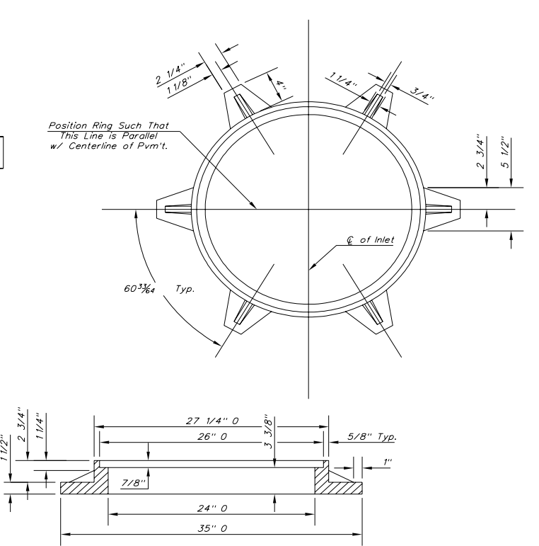
MANHOLE RING AND COVER
