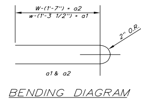
BENDING DIAGRAM
